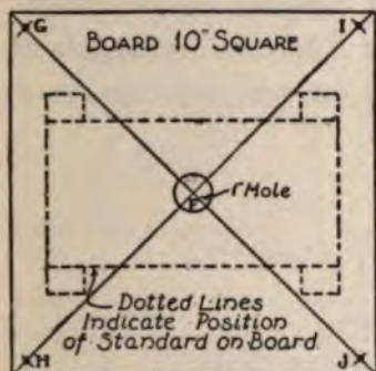
FIG. 140. — Plan of Top of Standard for Merry-go-round.
